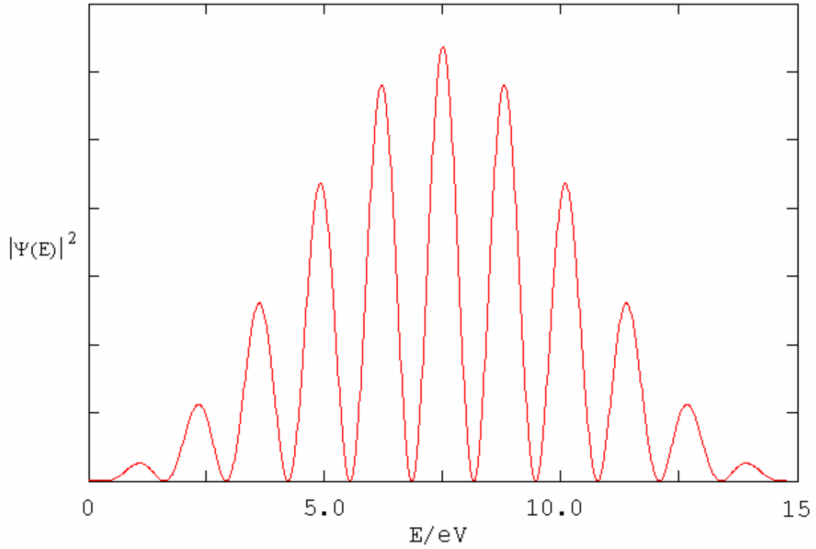
Figure 2. Relative electron kinetic energy distribution in eV. Estimating from reference [1] that \Delta t = t_2 - t_1 = 2.9 fs and \delta = 500 as yields a 15 eV envelope showing 11 interference fringes.
